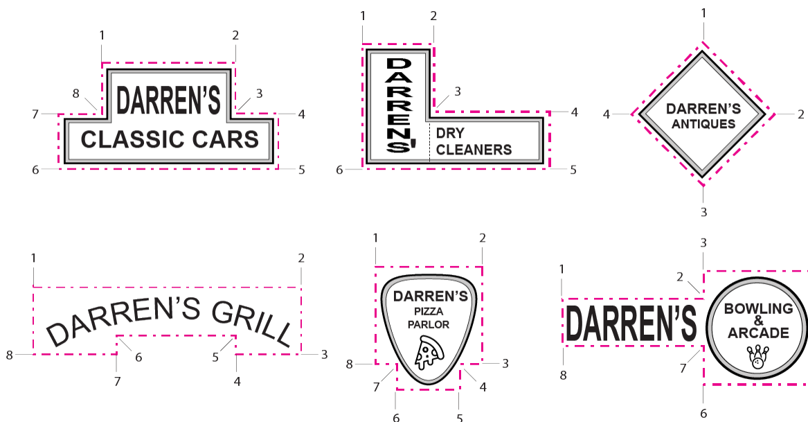
Figure 21.52.070-3 Calculating Sign Area – Single-Faced Signs
