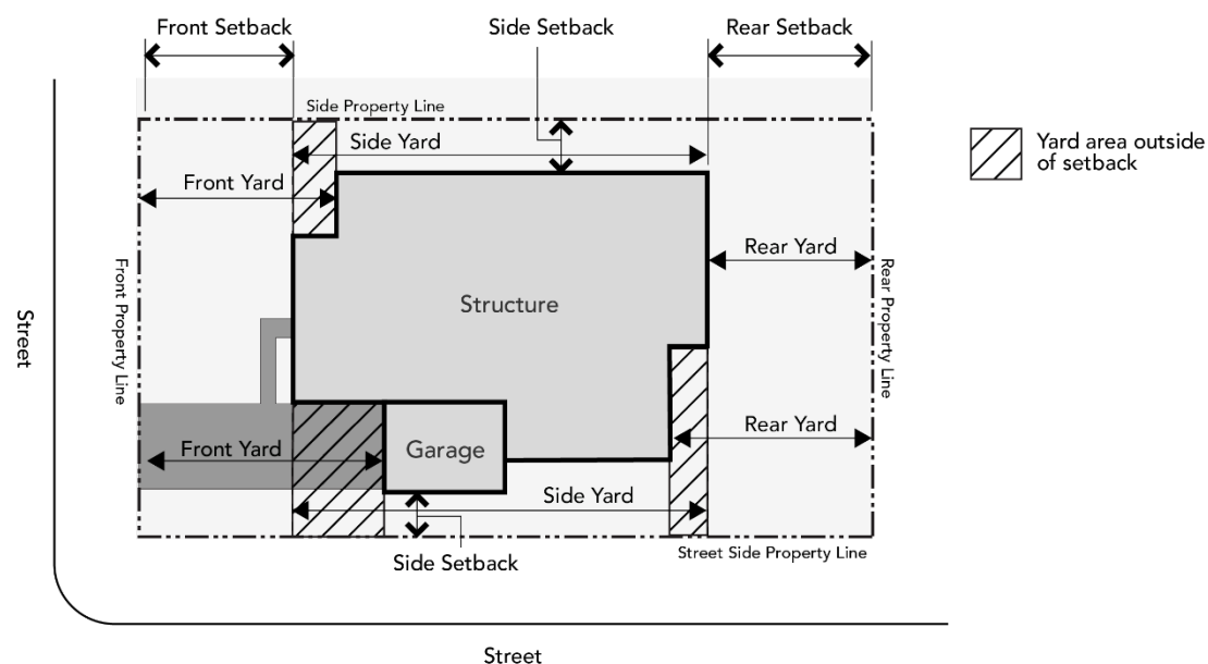
Figure 21.92.250-1: Yard Types
