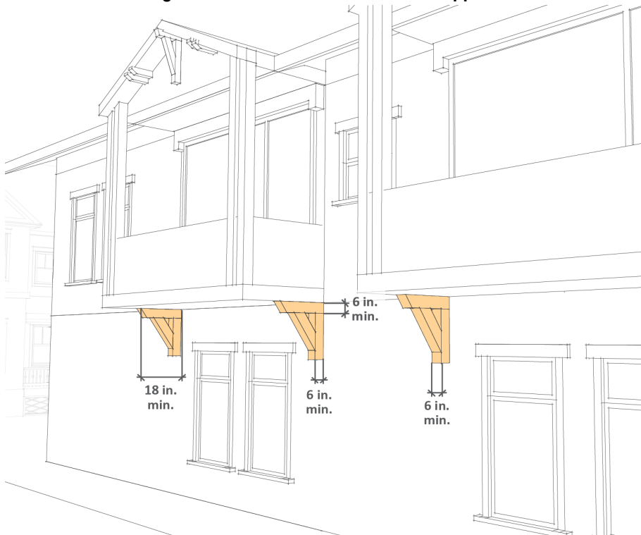
Figure 21.50.050-7: Post and Beam Supports
